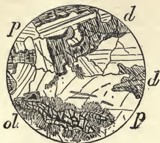
Fig. 30.—Olivine-Gabbro. Near Huntly, Aberdeen. \times 7 . d , Diopside, with numerous inclusions developed by schillerisation. On its margins it is passing by further change into brown strongly pleochroic hornblende, as indicated by the darker bands. ol , Olivine with fibrous marginal zone at contact with the felspars (development of actinolitic and other amphiboles; "dynamo-metamorphic" zone of Rosenbusch). p , Large crystals of plagioclase.
